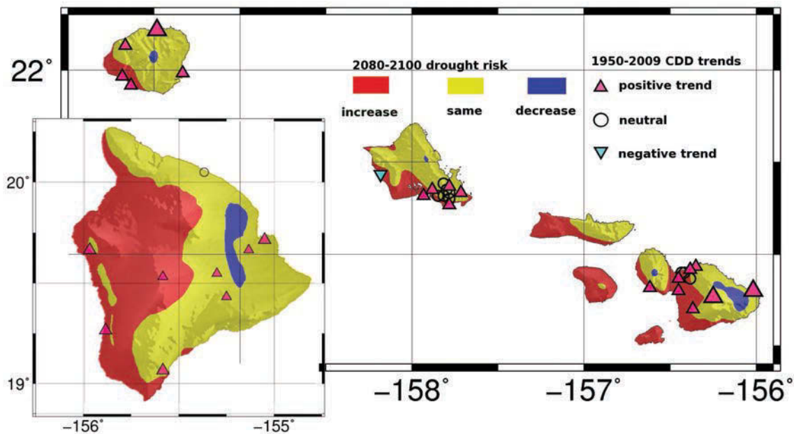
Figure 2-16 All four major Hawaiian Islands (O’ahu, Kaua’i, Maui, and Hawai’i Island) have experienced increasing winter drought since the 1950s, defined by a longer annual maximum number of consecutive dry days. Background colors highlight changes in the number of low-precipitation months during the wet season (November–April) based on statistically downscaled climate change scenarios from six models of the IPCC AR4 report for years 2080–2100. (Figure courtesy of Oliver Elison Timm.)
