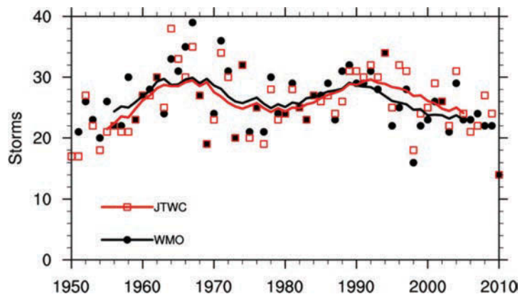
Figure 2-13 The number of tropical cyclones in the WNP basin as observed by the World Meteorological Organization (WMO; black lines/dots) and the Joint Typhoon Warning Center (JTWC; red lines/dots) since 1950. Lines indicate smoothed storm trend. There are regular cycles of greater and lesser annual storm numbers, and there were only 14 named storms in 2010. (From Knapp et al. [2010] by permission of American Meteorological Society. Data from the International Best Track Archive for Climate Stewardship [IBTrACS].)
