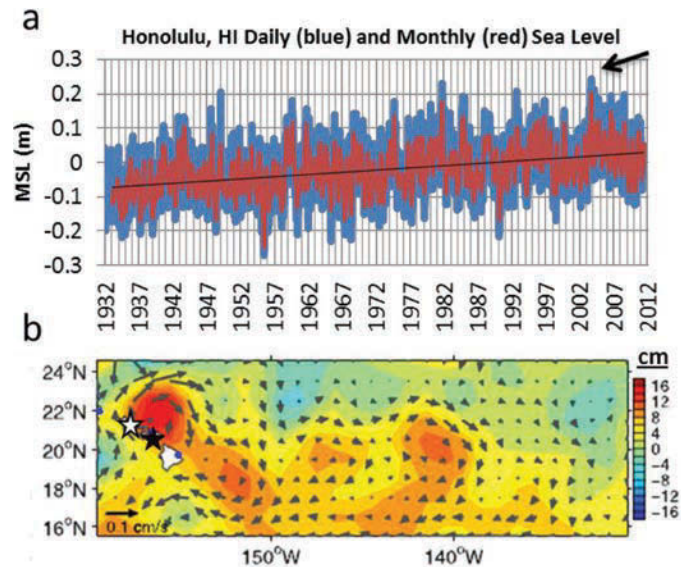
Figure 3-15 (a) Daily and monthly mean sea levels at NOAA Tide Gauge Honolulu (white star in (b)) are shown relative to the 1983–2001 mean sea level (MSL). The black line indicates the long-term relative sea-level rise (about 1.5 mm [0.059 in]/year); the arrow indicates the September 2003 event. (b) The gridded altimeter sea-surface height (SSH, contours in centimeters (cm), and mean circulation (vectors) for August 7, 2003, reveals the eddy directly north of the Hawaiian Islands. 0.1 m = 10 cm = 3.94 in. (Data in Figure 3-15a from NOAA; Figure 3-15b © 2004 American Geophysical Union. Reproduced/modified from Firing & Merrifield [2004] by permission of American Geophysical Union.)
