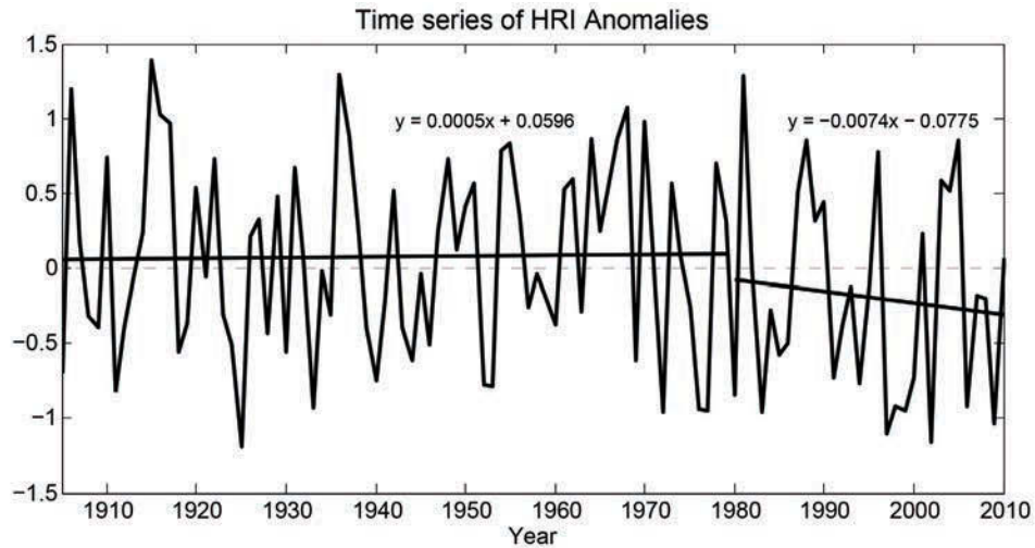
Figure 2-5 Annual normalized and dimensionless (July to June) time series of the Hawai'i Rainfall Index (HRI) from 1905 to 2010. As shown in the plot, the trend for the first epoch (1905–1979) is basically flat, while for the second epoch (1980–2009) the decreasing trend is apparent. Nine stations each from Kaua'i, O'ahu, and Hawai'i are used. These 27 stations represent the spatial variability of rainfall with regard to trade wind exposure and elevation. (Updated from Chu & Chen, 2005.)
