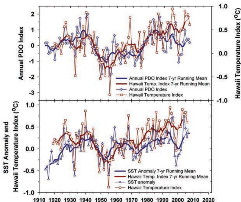
Figure 2-4 TOP PANEL—Air Temperature in Hawai‘i (red line) prior to 1975 is tightly coupled to the Pacific Decadal Oscillation (PDO) (blue line). Since 1975, air temperature (red line) has diverged increasingly from the observed PDO, which may indicate the increasing influence of climate change in the Central North Pacific sub-region. BOTTOM PANEL—Local sea-surface temperature anomalies (blue line) for 22°N, 156°W based on the Extended Reconstructed Sea-Surface Temperatures (ERSST) data set (Smith & Reynolds, 2004) are also coupled to air temperatures (red line) in Hawai‘i and show a similar decoupling around 1975. (©2008 American Geophysical Union. Reproduced/modified from Giambelluca et al. [2008] by permission of American Geophysical Union.)
