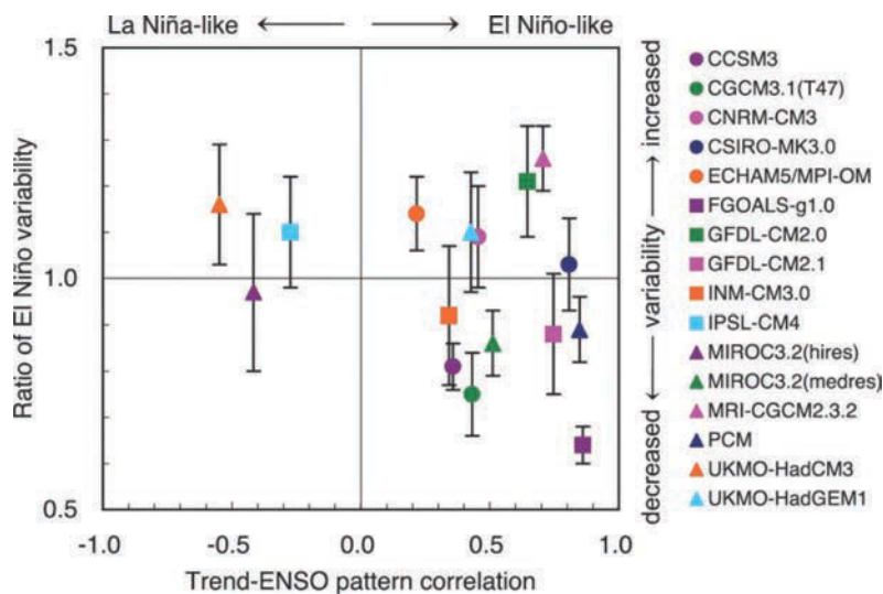
Figure B-4 Base state change in average tropical Pacific SSTs and change in El Niño variability simulated by AOGCMs. The base state change (horizontal axis) is denoted by the spatial anomaly pattern correlation coefficient between the linear trend of SST in the 1\% \text{ yr}^{-1} \text{ CO}_2 increase climate change experiment and the first Empirical Orthogonal Function (EOF) of SST in the control experiment over the area 10^\circ\text{S} to 10^\circ\text{N} , 120^\circ\text{E} to 80^\circ\text{W} (reproduced from Yamaguchi and Noda, 2006). Positive correlation values indicate that the mean climate change has an El Niño-like pattern, and negative values are La Niña-like. The change in El Niño variability (vertical axis) is denoted by the ratio of the standard deviation of the first EOF of sea-level pressure (SLP) between the current climate and the last 50 years of the SRES A2 experiments (2051–2100), except for FGOALS-g1.0 and MIROC3.2(hires), for which the SRES A1B was used, and UKMO-HadGEM1, for which the 1\% \text{ yr}^{-1} \text{ CO}_2 increase climate change experiment was used, in the region 30^\circ\text{S} to 30^\circ\text{N} , 30^\circ\text{E} to 60^\circ\text{W} with a five-month running mean (reproduced from van Oldenborgh et al., 2005). Error bars indicate the 95% confidence interval. Note that tropical Pacific base state climate changes with either El Niño-like or La Niña-like patterns are not permanent El Niño or La Niña events, and all still have ENSO interannual variability superimposed on that new average climate state in a future warmer climate. (From IPCC AR4 Section 10.3.5.3, Figure 10.16; Meehl et al., 2007.)
