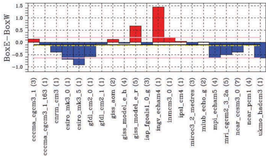
Figure B-5 The projected late 21st-century change in the difference in sea-level pressure between two boxes along the equator in the eastern and western Pacific in 21 CMIP3 models. The model identifiers are along the axis along with the number of realizations analyzed (in parentheses). (From Power & Kociuba, 2011.)
