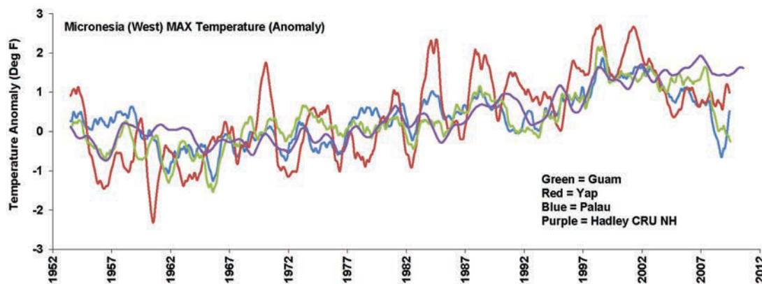
Figure 2-10 Maximum monthly temperature anomaly time series from 1952 to 2012 (using 1960–1990 as the mean reference period) for single monitoring stations with the most data in Yap, Guam, and Palau. The northern hemisphere temperature time series (purple line, Hadley CRU NH) is superimposed for comparison. Trends in maximum temperatures in the western part of the Western North Pacific sub-region appear to be increasing at the same general rate as average northern hemisphere temperatures, although Yap shows a high level of variability. (Updated from Lander & Guard, 2003.)
