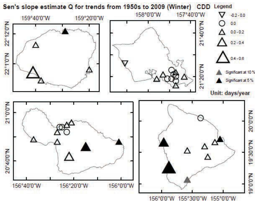
Figure 2-7 All four major Hawaiian Islands (O'ahu, Kaua'i, Maui, and Hawai'i Island) have experienced increasing winter drought severity since the 1950s, defined by a longer annual maximum number of consecutive dry days. Upward triangles denote the increasing drought trends, while downward triangles indicate decreasing trends. Black triangles are significant at the 5% level, and gray at the 10% level. (From Chu et al. [2010] by permission of American Meteorological Society.)
