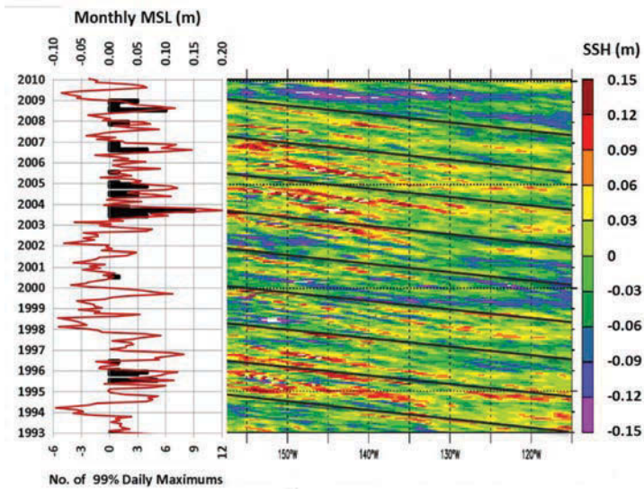
Figure 3-16 A time-longitude plot of SSH anomalies (right) along the altimeter track at 21.3°N shows that when high monthly mean sea levels at Honolulu (left, right line) are recorded, they often appear to originate further east along the same latitude range (right, eddies as red contours moving westward over the x-axis as time progresses on the left y-axis). 0.1 m = 0.33 ft. (©2004 American Geophysical Union. Reproduced/modified from Firing & Merrifield [2004] by permission of American Geophysical Union.)
