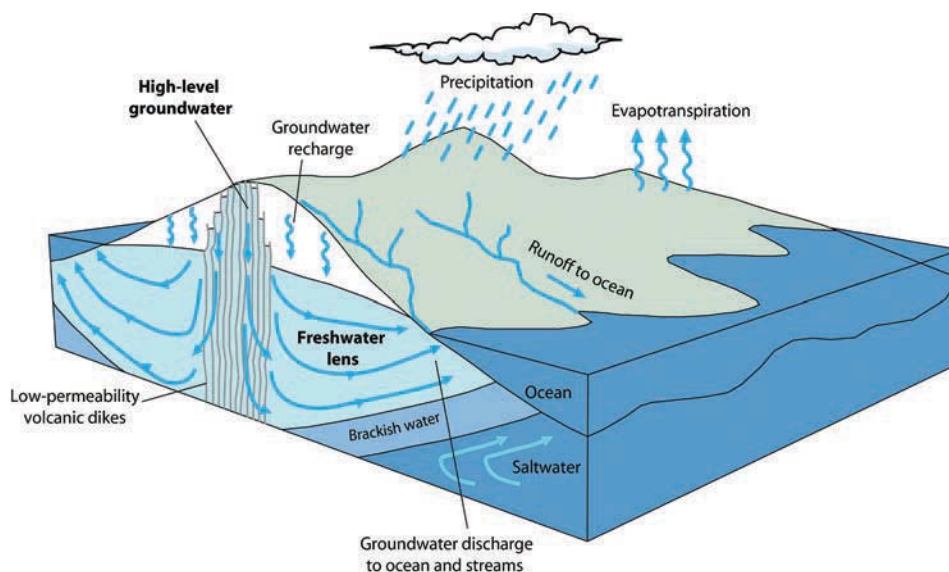
Figure 2-1 Cross section of regional hydrological processes. Precipitation is the source of both surface water, such as streams, and groundwater on Pacific Islands. Variations in precipitation and evapotranspiration rates therefore affect both resources. Surface water is important for human use and provides habitats for fragile ecosystems. Groundwater in islands exists as a freshwater lens underlain by saltwater, and on high volcanic islands it may also exist as high-level groundwater. Groundwater is a principal source of drinking water on high islands. (Modified from Izuka, 2011.)
