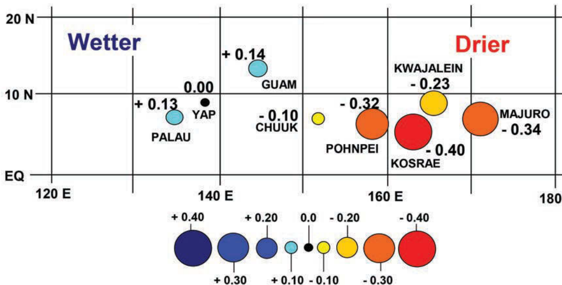
Figure 2-12 Annual rainfall anomaly (inches per month per decade) in the WNP sub-region from 1950 to 2010 shows that whereas islands in the west are tending toward getting slightly more precipitation, islands in the east are experiencing much less precipitation. Darker blue shading indicates wetter conditions, and darker red shading indicates drier. The size of the dot is proportional to the size of the trend as per the inset scale. (Modified and updated from Lander & Guard, 2003, and Lander, 2004.)
