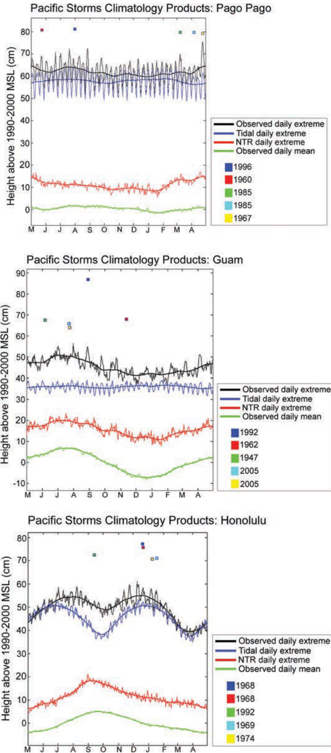
Figure 3-8 Extreme climatologies from tide gauges for each day of the year at selected tide stations in the Pacific (black, darker line is smoothed). The contribution to the extreme levels from the tides (blue), seasonal (green), and nontidal residual (red) are depicted. The five largest extreme events on record are also shown. Long-term linear trends in time series have been removed. Note how in Pago Pago (top), extremes are governed by the seasonal tidal signal. In contrast, in Guam (middle), it is the seasonal occurrence of tropical cyclones that dominates extremes. In Honolulu (bottom), there is both a tidal and a storm component in the signal. (From NOAA NCDC at http://www.pacificstormsclimatology.org/ .)
