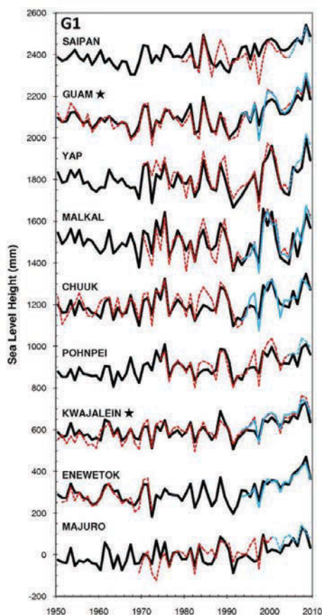
Figure 3-3 Sea-level time series (red) at Pacific Island tide-gauge sites, including reconstructed time series (black) and altimeter sea levels (blue). Note high interannual variability and the recent upward trend since the mid-1990s. (From Becker et al. [2012] by permission of Elsevier.)
