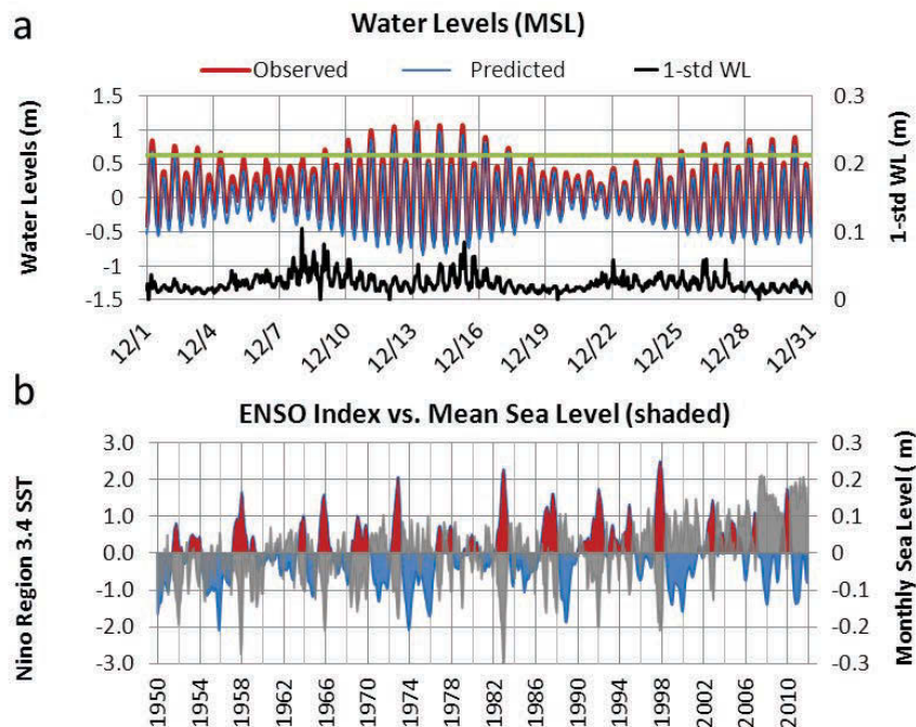
Figure 3-13 In mid-December 2008, the Marshall Islands experienced high seasonal spring (king) tides causing water levels to rise above the Mean Higher High Water (MHHW, green) level. Around this time (a) multi-day periods with enhanced wave activity and related swash motions at the shoreline occurred ~ Dec 8 and 15 seen as high variability within each hourly water-level measurement (1-std WL, Sweet et al., 2011). In (b), the ENSO Niño Region 3.4 anomaly (red/blue) shows elevated sea levels during cool phase/La Niña (blue) or warm phase/El Niño (red), which have steadily increased since about 1990. 0.1 m = 0.33 ft. (Data from NOAA Tide Station at Kwajalein, Marshall Islands.)
