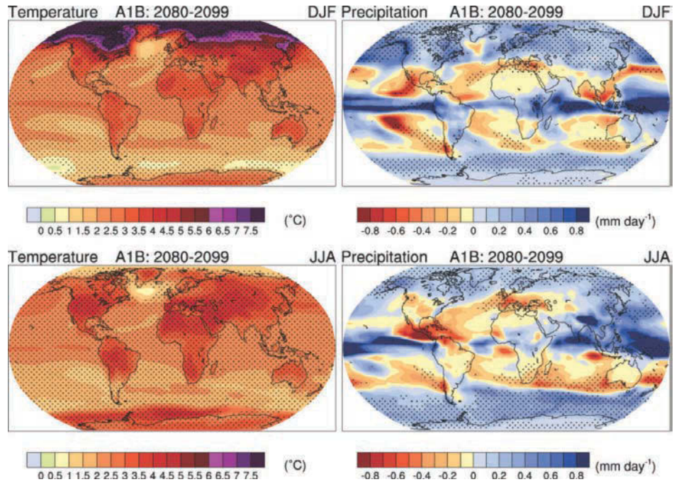
Figure B-6 The change over the 21st century in surface air temperature (left) and precipitation (right) in the multi-model ensemble of CMIP3 SRESA1B integrations. Results for December–February (top) and June–August (bottom). Stippling indicates where the magnitude of the multi-model mean change exceeds the inter-model standard deviation. From AR4. (From IPCC AR4 Section 10.3.2.1, Figure 10.9; Meehl et al., 2007.)
