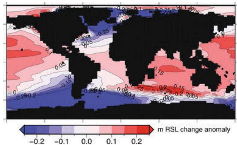
Figure 3-10 Local relative sea-level (RSL) change anomaly with respect to global mean change estimates (1.02 m:3.35 feet) between 1980–1999 and 2090–2099 based on an ensemble of coupled climate model simulations for the IPCC A1B emission scenario (IPCC, 2007) with an adapted ice-sheet contribution of 0.22 m (0.72 feet) for Greenland and 0.41 m (1.35) from Antarctica. (From Slangen et al., 2011.)
