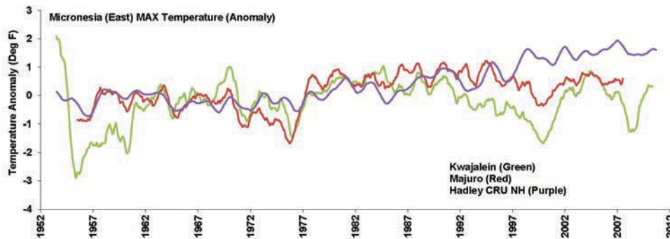
Figure 2-11 Maximum monthly temperature anomaly time series from 1952 to 2012 (using 1960–1990 as the mean reference period) for single monitoring stations with the most data in Kwajalein and Majuro in the RMI. The northern hemisphere temperature time series (purple line, Hadley CRU NH) is superimposed for comparison. Trends in maximum temperatures in the eastern part of the Western North Pacific sub-region have high levels of variability and may reflect issues in the quality of the data or station infrastructure. (Modified and updated from Lander & Guard, 2003.)
