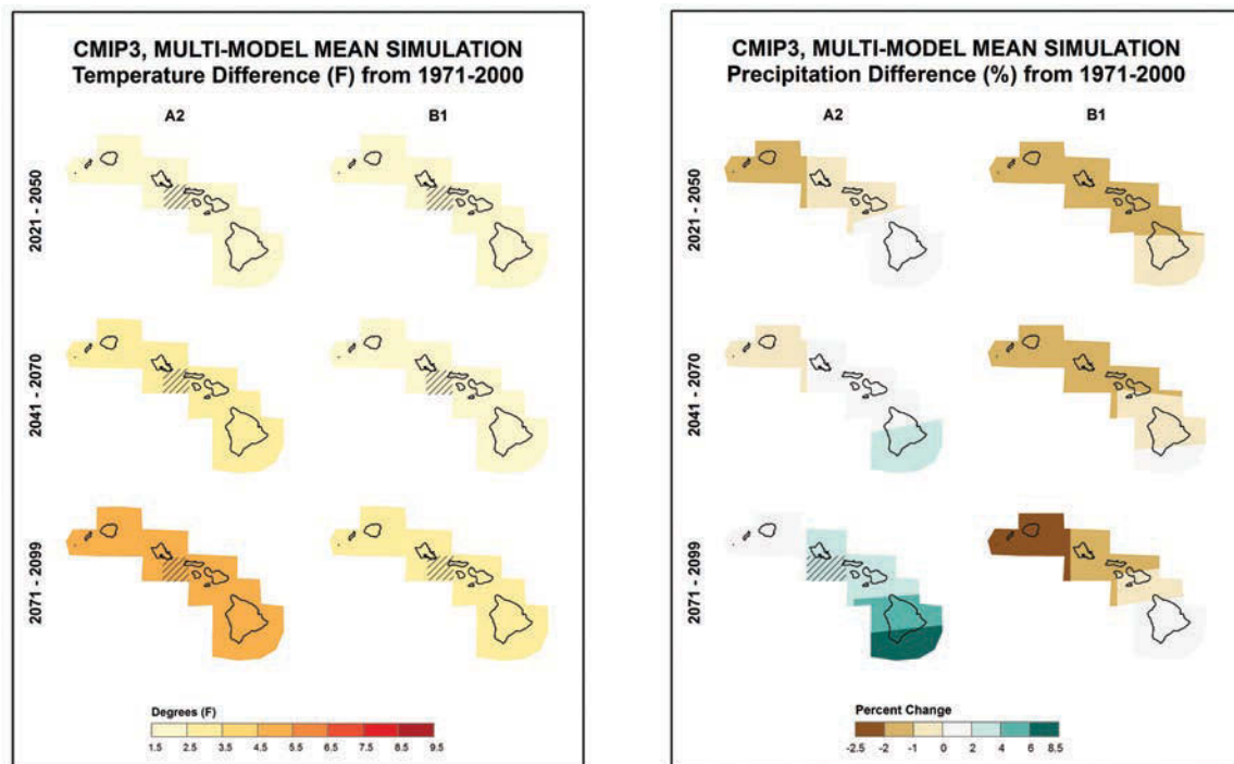
Figure 1-8 Multi-model mean annual differences in (left) temperature (°F) and (right) precipitation (%) in Hawai'i between the three future periods and 1971–2000, from the 15 CMIP3 model simulations. (Courtesy of Ken Kunkel, NOAA NCD and North Carolina State University.)
