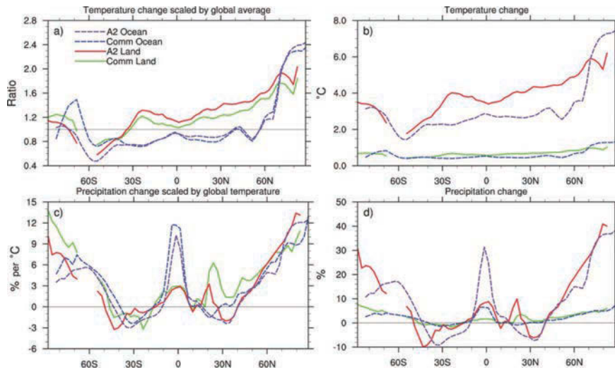
Figure B-1 The general magnitude of changes in air temperature and precipitation in the Pacific region is projected to be comparable to global estimates of average change over both land and ocean. Zonal means over land and ocean separately, for annual mean surface warming (a, b) and precipitation (c, d), shown as ratios scaled with the global mean warming (a, c) and not scaled (b, d). Multi-model mean results are shown for two scenarios, A2 and Commitment, for the period 2080–2099 relative to the zonal means for 1980–1999. (From IPCC AR4, Section 10.7, Figure 10.6; Meehl et al., 2007.)
