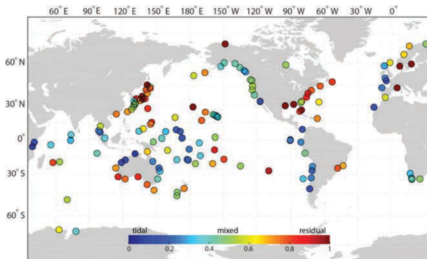
Figure 3-6 The ratio of mean nontidal residual to mean extreme amplitude for annual maxima. (©2012 American Geophysical Union. Reproduced/modified from Merrifield et al. [2012] by permission of American Geophysical Union.)
