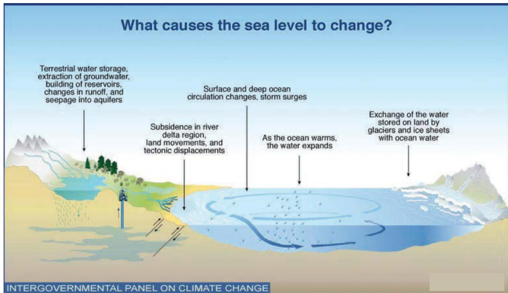
Figure 3-2 Causes of sea-level change. (From IPCC, 2001.)
