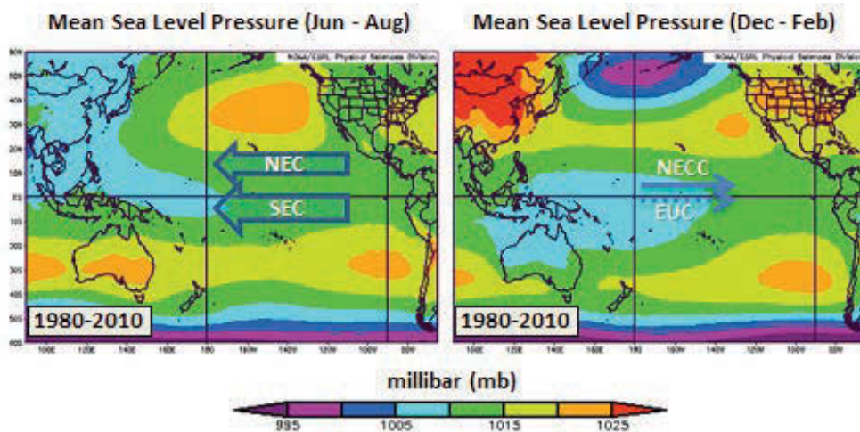
Figure 1-3 Northern hemisphere summer (June–August) versus winter (December–February) plots of the annual average atmospheric pressure at sea level (SLP). In June–August (left), the area of strong average high pressure (orange) that extends across the CNP corresponds to the NPH. In December–February (right), the area of strong average low pressure (purple) centered on the Gulf of Alaska corresponds to the AL. (Courtesy of NOAA ESRL Physical Sciences Division.)
