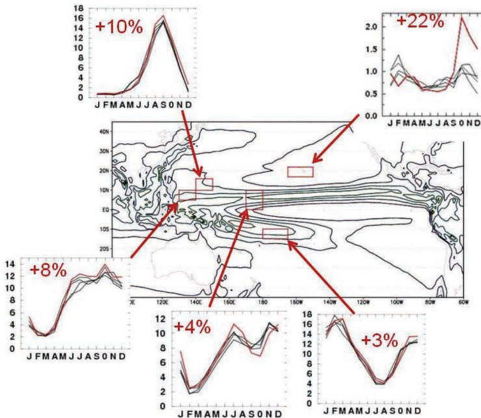
Figure B-7 CMIP5 climate change results from the Hadley Centre HADGEM2-ES model. Shown are the mean annual cycle of precipitation averaged over five individual boxes corresponding to the locations of the major groups of USAPI. Results for the late 20th century from the CMIP5 “Historical” simulation (black curves) and for the late 21st century from a RCP4.5 climate change projection simulation (red curves). Each curve represent results from 20 years of simulation. Results from four 20th-century ensemble members and from a single RCP4.5 realization. The red numbers indicate the percentage change of annual mean precipitation in the RCP4.5 results relative to the late 20th-century simulations. (Figure courtesy of Kevin Hamilton.)
