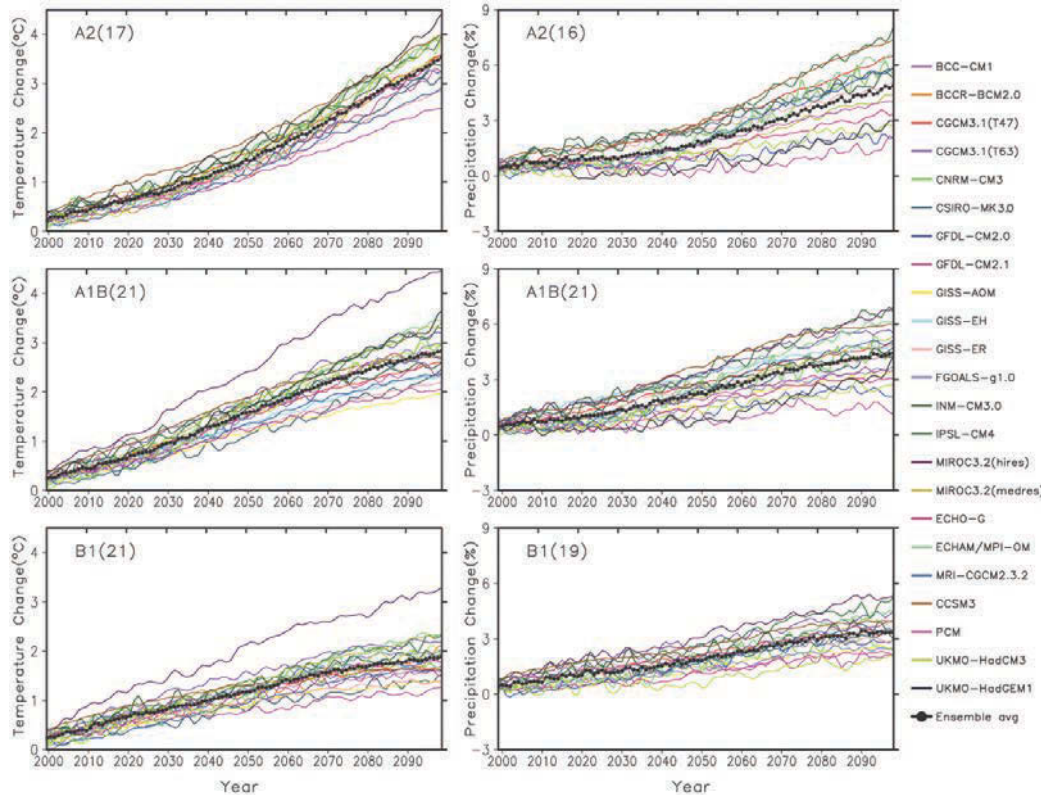
Figure B-3 Time series of globally averaged (left) surface warming (surface air temperature change, °C) and (right) precipitation change (%) from the various global coupled models for the scenarios A2 (top), A1B (middle), and B1 (bottom). Numbers in parentheses following the scenario name represent the number of simulations shown. Values are annual means, relative to the 1980–1999 average from the corresponding 20th-century simulations, with any linear trends in the corresponding control-run simulations removed. A three-point smoothing was applied. Multi-model (ensemble) mean series are marked with black dots. (From IPCC AR4, Section 10.3.1, Figure 10.5; Meehl et al., 2007.)
