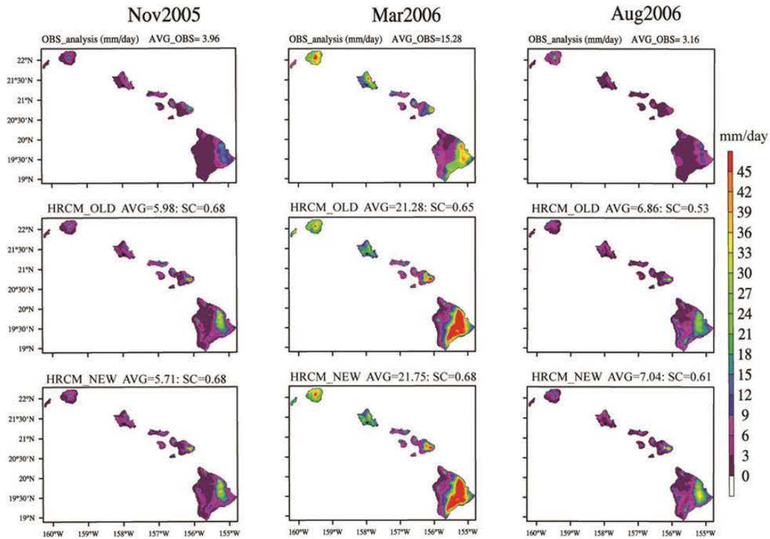
Figure B-8 Monthly rainfall over the main Hawaiian Islands from a one-year simulation with the regional WRF-ARW model modified as described in Zhang et al. (2012). Results from two versions of the model are shown in the middle and lower rows. Observations in the top row are objective analyses based on rain-gauge observations at a large number of stations. Results for November 2005, March 2006, and August 2006 are shown.
