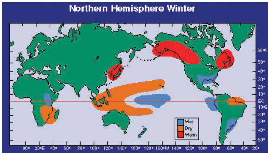
Figure 1-5 Precipitation during El Niño in the northern hemisphere winter. (Courtesy of NOAA Pacific Marine Environmental Laboratory.)
