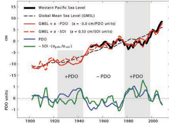
Figure 3-5 Western Pacific sea level (black) compared to reconstructions based on the PDO (red) and the SOI (red dash) with the Church and White (2011) global mean sea level included (black dash). The PDO index (blue) and scaled SOI (green) are shown for comparison. (©2012 American Geophysical Union. Reproduced/modified from Merrifield et al. [2012] by permission of American Geophysical Union.)
