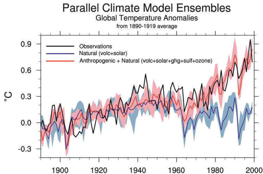
Figure 1-6 Simulated natural versus human-induced global temperature, 1890–2000. Using an ensemble of four climate models, scientists can differentiate between human-induced trends and natural trends in long-term global climate variables. Here, the observed change in global annual air temperature (black line) is compared to the predicted range of air temperature with only natural climate variability (blue line with blue shading) and the predicted range with both natural plus human-induced factors (red line with pink shading). Natural factors include volcanic and solar activity, while human-induced activity adds the effects of greenhouse gases, sulfates, and ozone (Meehl et al., 2009). In the Pacific region, high ENSO-related variability makes it more difficult to separate the long-term and short-term trends. (From Meehl et al. [2009] by permission of American Meteorological Society.)
