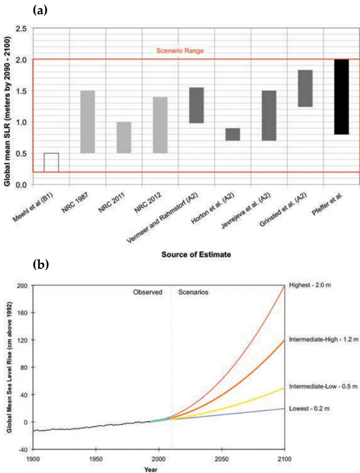
Figure 3-9 (a) End-of-century (~2090–2100) estimates for global mean sea level rise in meters. Meehl et al. (2007) is based on climate model projections for the IPCC and outlined in black. NRC (1987, 2011, and 2012) is based on synthesis of the scientific literature and shown in light gray. Vermeer and Rahmstorf (2009), Horton et al. (2008), Jevrejeva et al. (2010), Grinsted et al. (2009) are based on semi-empirical approaches and shown in dark gray. Pfeffer et al. (2008) is a calculation of the maximum possible contribution from ice sheet loss and glacial melting and shown in black. (b) Global mean sea level rise scenarios developed for the 2013 NCA. Present mean sea level (MSL) for the US coasts is determined from the National Tidal Datum Epoch (NTDE) provided by NOAA. The NTDE is calculated using tide gage observations from 1983–2001 and 1992, the mid-point of the NTDE, is chosen as a starting point. (From Parris et al., in press).
