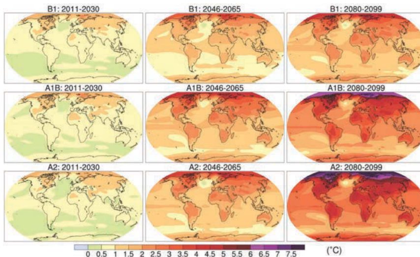
Figure B-2 Global-scale temperature patterns for three IPCC warming scenarios and time periods are shown here. In each case, greater warming over most land areas is evident. Over the ocean, warming is relatively large in the Arctic and along the equator in the eastern Pacific. Multi-model mean of annual mean surface warming (surface air temperature change, °C) for the scenarios B1 (top), A1B (middle), and A2 (bottom), and three time periods, 2011–2030 (left), 2046–2065 (middle), and 2080–2099 (right). Anomalies are relative to the average of the period 1980–1999. (From IPCC AR4, Section 10.3.2.1, Figure 10.8; Meehl et al., 2007.)
