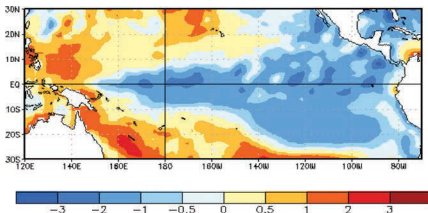
Figure 2-17 The NOAA Climate Prediction Center (CPC) released a seasonal ENSO outlook indicating La Niña conditions, or colder-than-average sea-surface temperatures in the equatorial Pacific Ocean. Here, in December 2010, the plume of cold (blue) water is visibly extending westward along the equator. (Courtesy of NOAA CPC, “December 2011 Sea-surface Temperatures.”)
