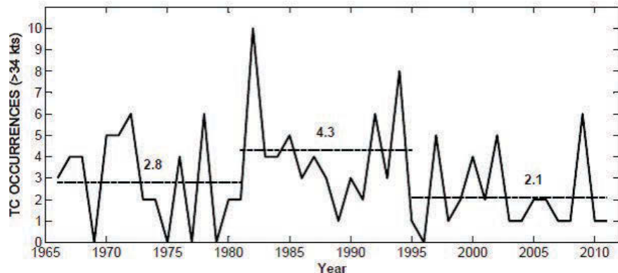
Figure 2-6 Time series of tropical cyclones (tropical storms and hurricanes) in the Central North Pacific basin from 1966 to 2010. Although a period of greater tropical cyclone activity occurred from the 1980s to the mid-1990s, the basin has again entered a quieter period, with fewer average annual occurrences of storms. Broken lines denote the means for the periods 1966–1981, 1982–1994, and 1995–2010. (Modified and updated from Chu, 2002.)
