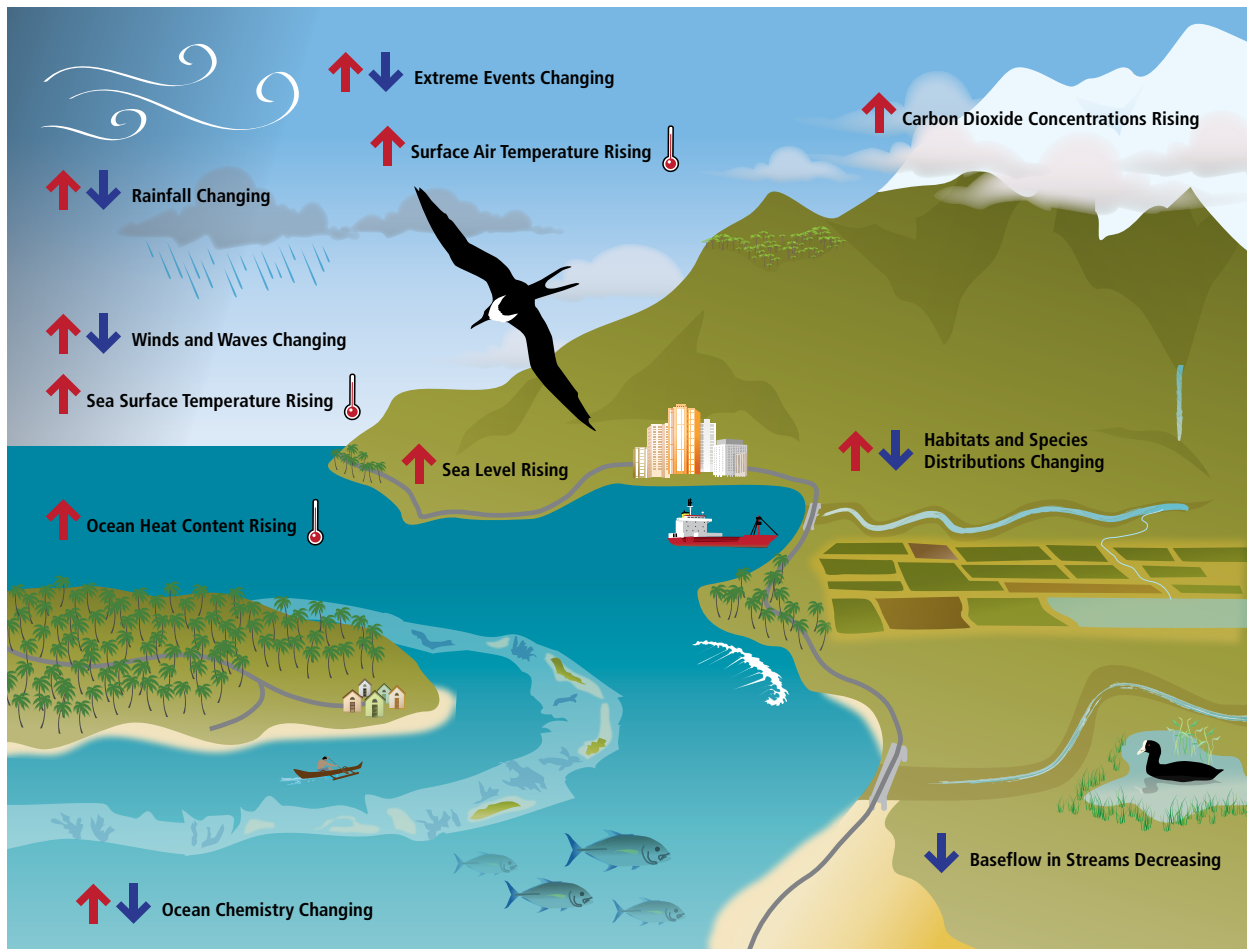
Figure 1-9 Indicators of climate change in the Pacific Islands region. (Courtesy of Susan Yamamoto, Geovision. Adapted from "Ten Indicators of a Warming World," in NOAA National Climatic Data Center, State of the Climate 2009 [report].)
