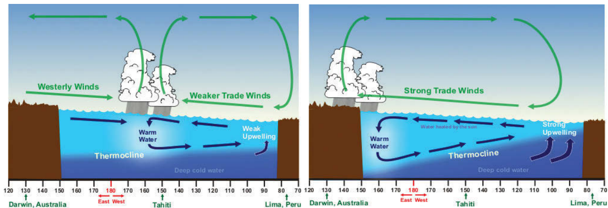
Figure 1-4 El Niño and La Niña events. During El Niño (left), the trade winds decrease, ocean water piles up off South America, the SST increases in the eastern Pacific, and there is a shift in the prevailing rain pattern from the western Pacific to the western Central Pacific. During La Niña (right), the trade winds increase, ocean water piles up in the western Pacific, the SST decreases in the eastern Pacific, and the prevailing rain pattern also shifts farther west than normal. (Courtesy of NOAA National Weather Service.)
