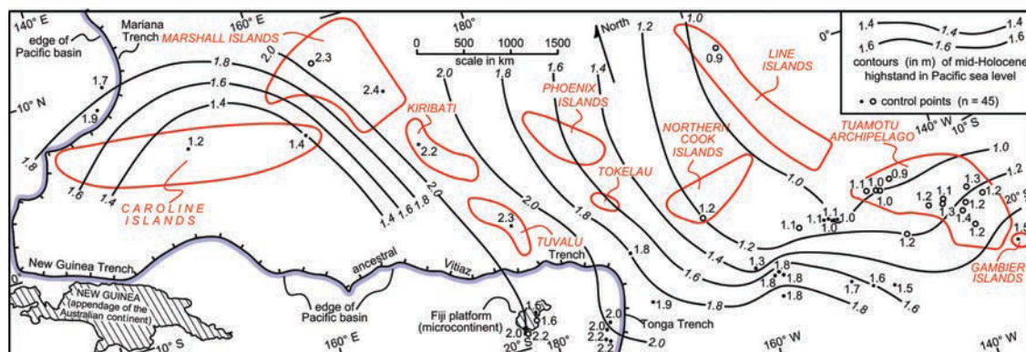
Figure 3-11 Contours of the magnitude (above modern sea level) of the hydro-isostatic mid-Holocene highstand in regional sea level across the tropical Pacific Ocean; solid dots are control points (number [n] = 27) from personal observations (Dickinson, 1998, 1999, 2000, 2001, 2003; Dickinson et al., 1999; Dickinson & Burley, 2007), and open dots are congruent control points (n = 18) from others (Pirazzoli & Montaggioni, 1986, 1988; Nunn, 1988, 2000; Woodroffe et al., 1990; Woodroffe & McLean, 1998; Grossman et al., 1998). For contouring, control points within the microcontinental Fiji platform were ignored from the perspective that isostatic upflexure of the platform under the enhanced load of deepening water offshore promoted emergence that partly counteracted SLR (Nakada, 1986). (From Dickinson, 2009.)
