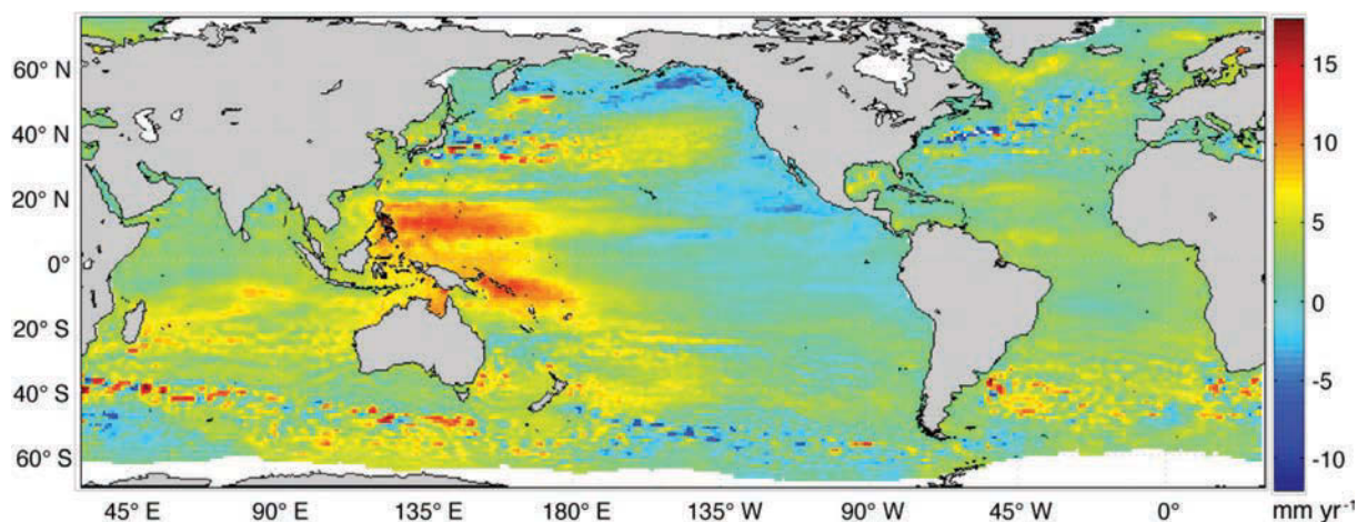
Figure 3-4 Sea-level trend for 1993–2010 from Aviso altimeter product, produced by Ssalto/Duacs with support from the Centre National d'Etudes Spatiales. (From Merrifield [2011] by permission of American Meteorological Society.)
