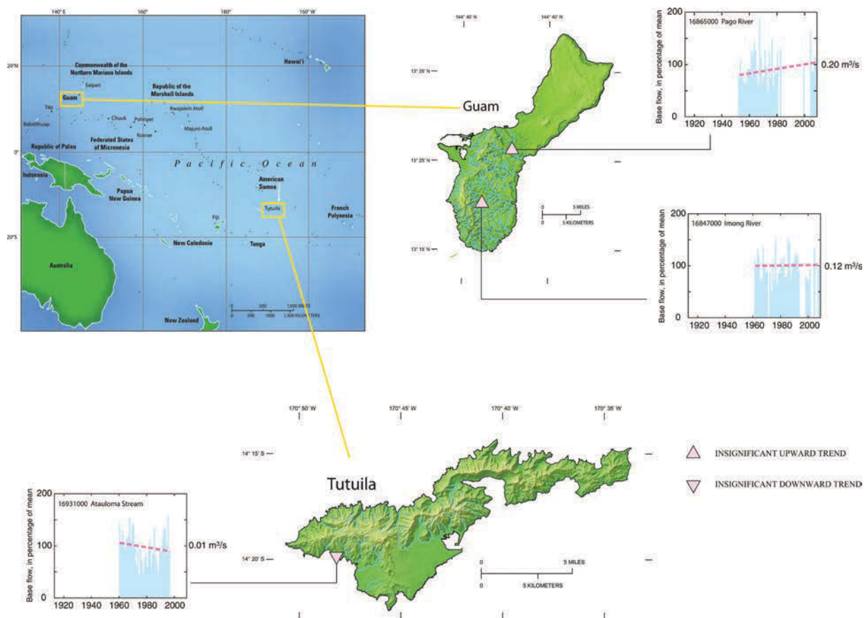
Figure 2-14 Streamflow records available for the Western North Pacific and Central South Pacific sub-regions are relatively short and mostly discontinuous, and many have been affected by upstream diversions or other human activities. Analysis of data from 1978 to 2008 from two gauges on Guam and one on Tutuila, American Samoa, showed no statistically significant trends (red dashed line) in the number of extreme high- or low-flow days. The lack of significant streamflow trends on Guam and American Samoa is consistent with rainfall observations but may also be an artifact of short record available for analysis, highlighting the need for consistent and high-quality monitoring in these sub-regions. (From Miller et al., 2012.)
