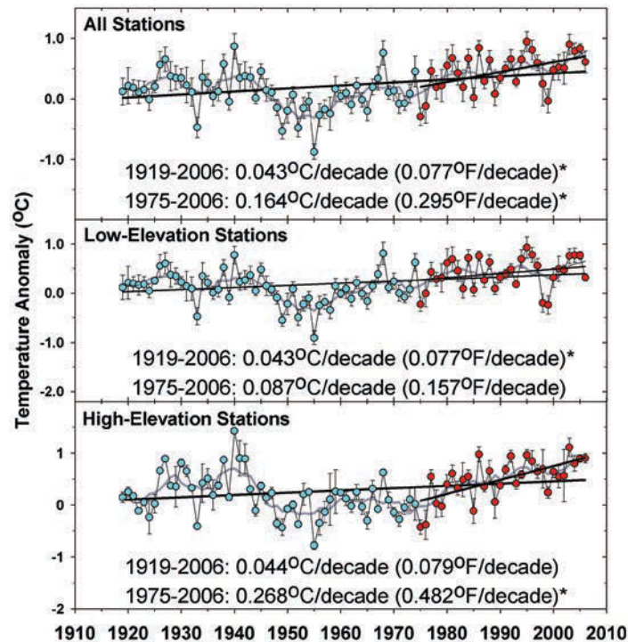
Figure 2-3 Annual average surface temperature anomalies are increasing at both high- and low-elevation stations in Hawai'i (a total of 21). Temperature anomalies are calculated first as the departure from the monthly mean and then averaged into a calendar year. Anomalies greater than zero indicate temperatures that are above average, while anomalies less than zero indicate below-average temperatures. A seven-year running-mean filter (curved line) has been applied to the data to create a smoothed trend curve (black line). Linear trends have been computed for two periods, 1919–2006 and 1975–2006, where the latter period shows the observed enhanced warming. The steeper warming trend in high-elevation stations (>800 meters or >0.5 mile) is visible in the bottom panel, especially when compared to that of the low-elevation stations in the middle panel (<800 meters or <0.5 mile). Error bars show a standard deviation of +0.5. Asterisks indicate slopes significant at p = 0.05 . (© 2008 American Geophysical Union. Reproduced/modified from Giambelluca et al. [2008]) by permission of American Geophysical Union.)
